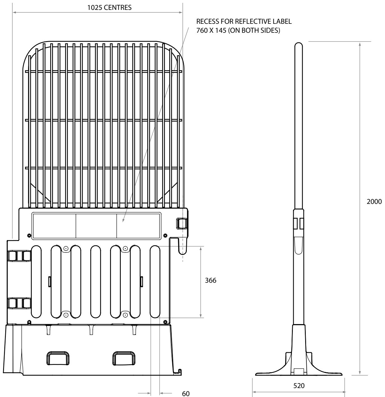
ASSEMBLED PRODUCT
